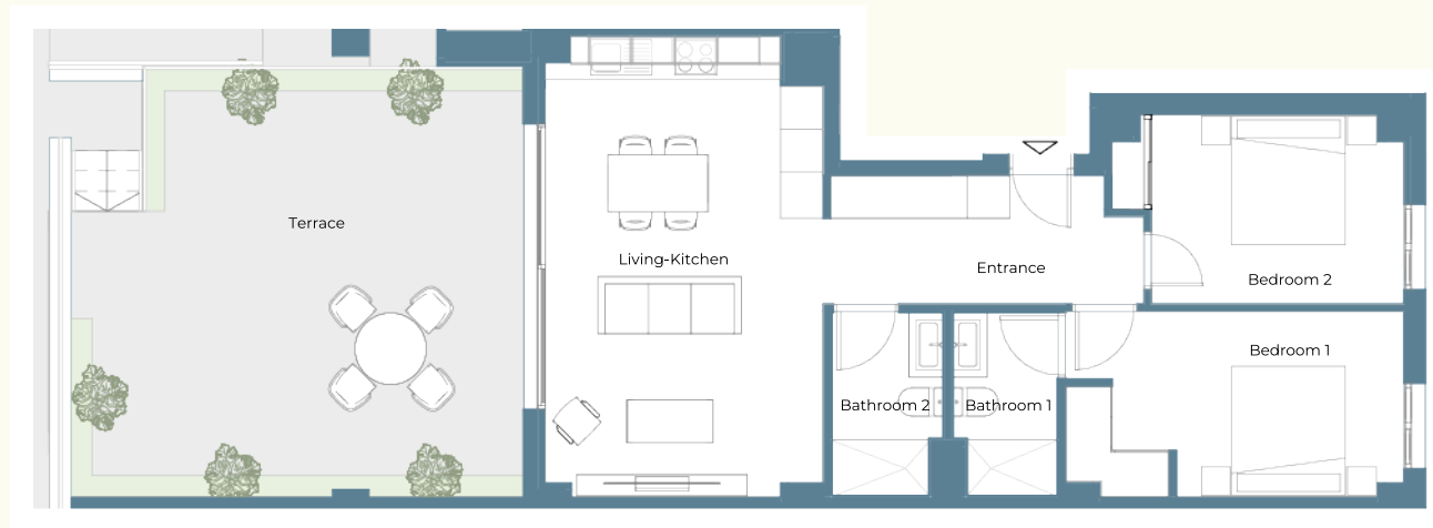
STANDARD GROUND FLOOR
